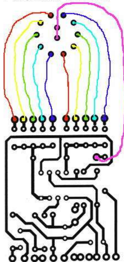
DPST WIRING FOR FREQUENCY BOOSTER
