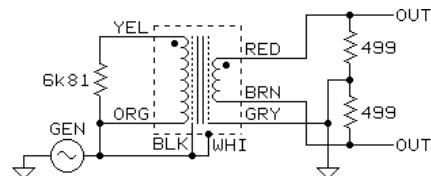
TEST CIRCUIT 2
