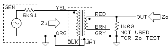
TEST CIRCUIT 1
