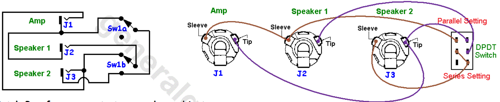
Patch Box for an amp to two speaker cabinets. Switchable for series or parallel connections.
